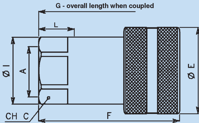
IACP SERIES PULL BREAK FEMALE COUPLING
