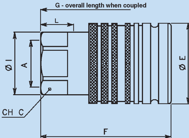
IACP SERIES PUSH PULL FEMALE COUPLING
