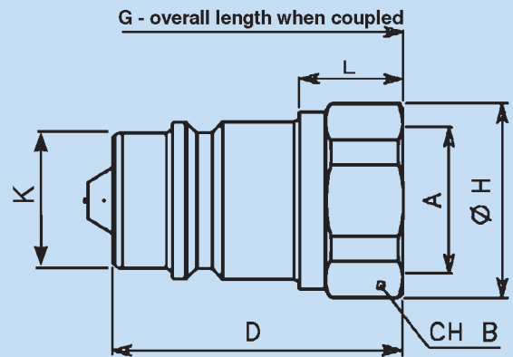
IACP SERIES MALE COUPLING
